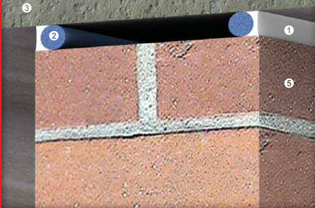
Typical head and control joints of masonry wall (STC 49)
