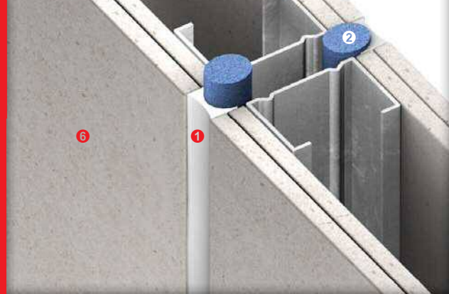
Typical control joints of lightweight partition (STC 45-50)
