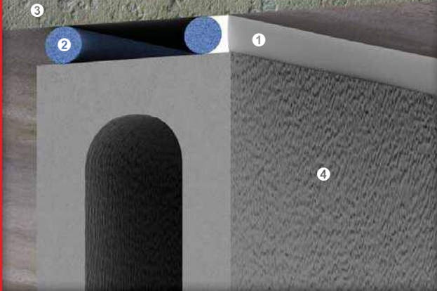
Typical head and control joints of concrete hollow block wall (STC 45)
